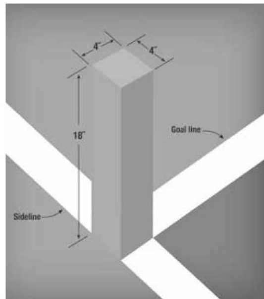
PYLON DETAIL
